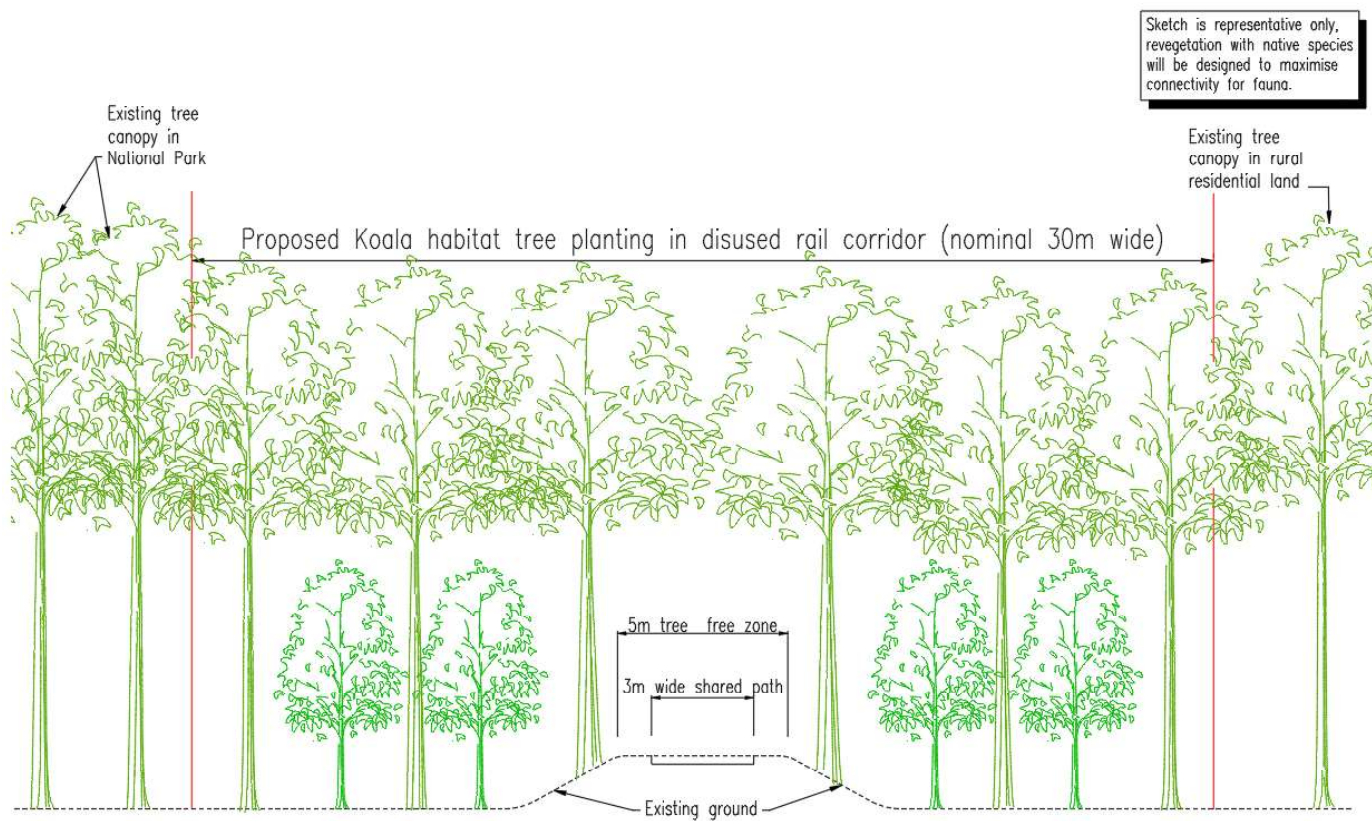
Figure 5 Rehabilitation of disused rail corridor near Beerburrum (indicative) (ARUP, 2020)
